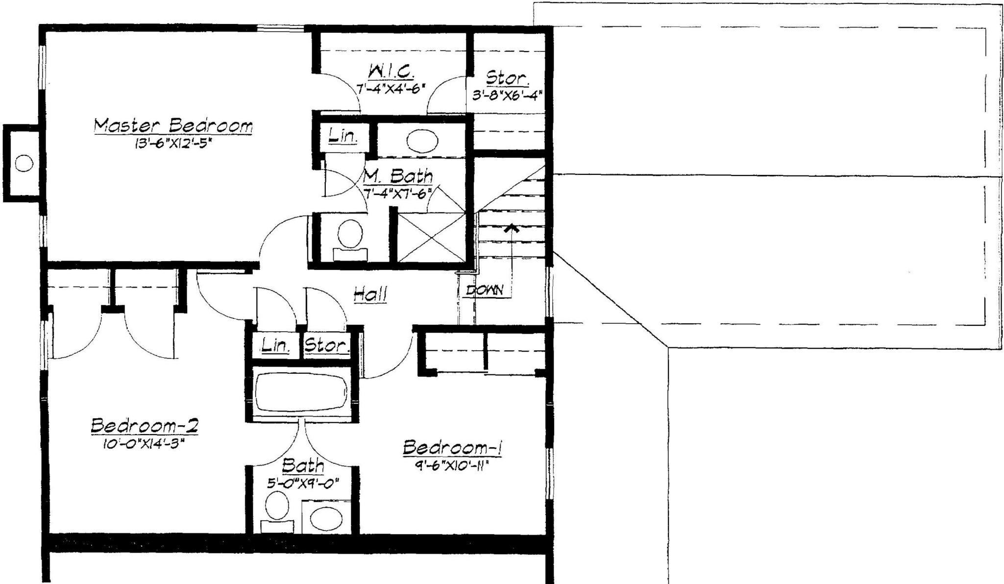
Typical Unit Second Floor Plan
